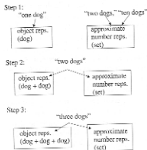
Figure 10.12 Hypothesized linkages between number words and core systems of representation at the first three steps in children's developing understanding of counting, number words, and the natural numbers
